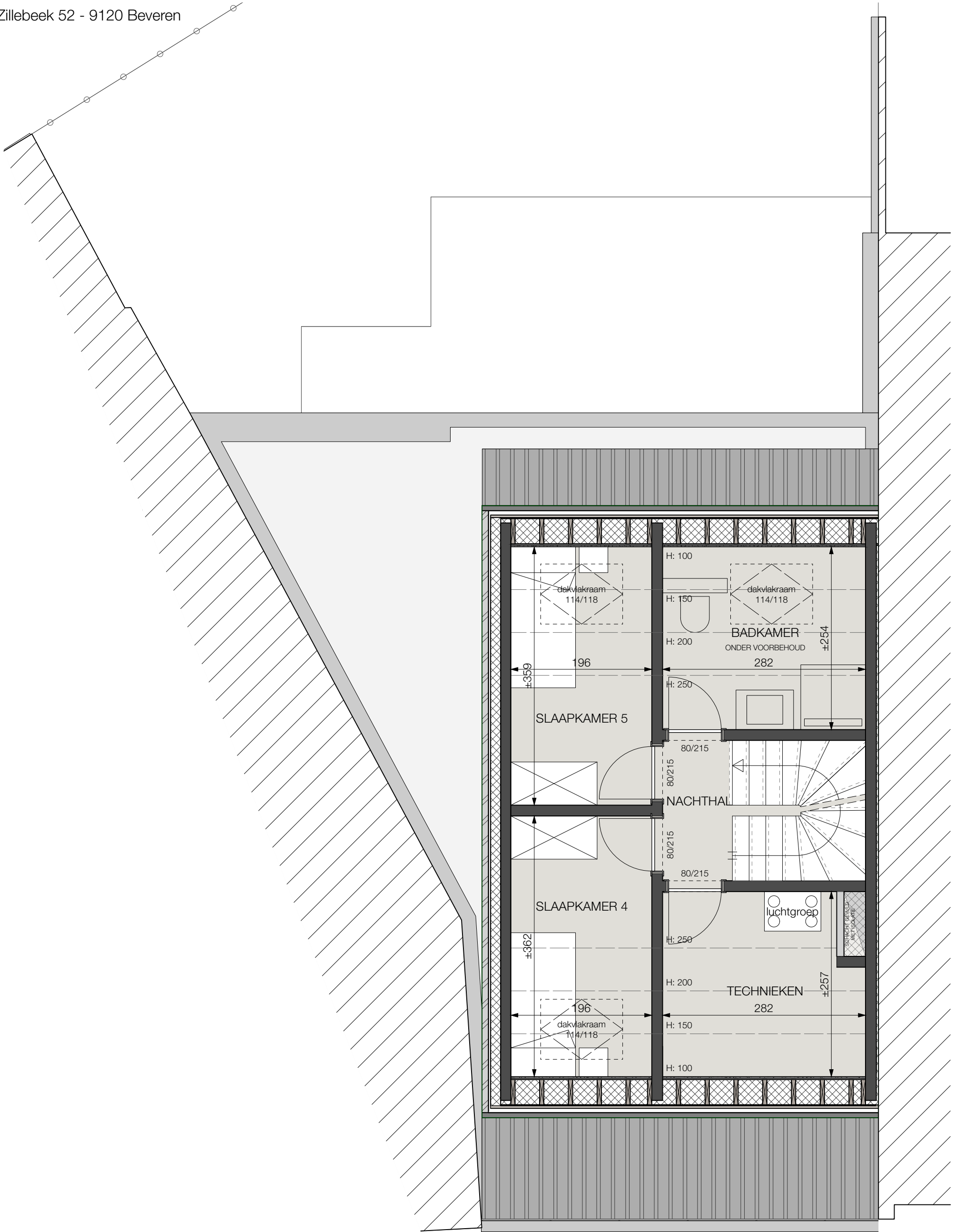
WONING 1: VERDIEPING +02
