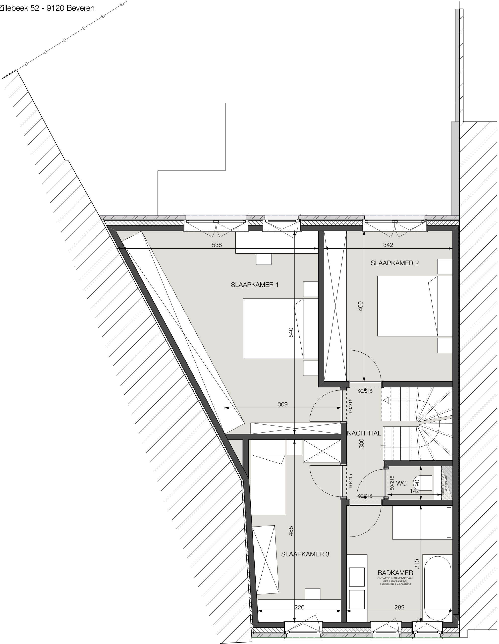
WONING 1: VERDIEPING +01
